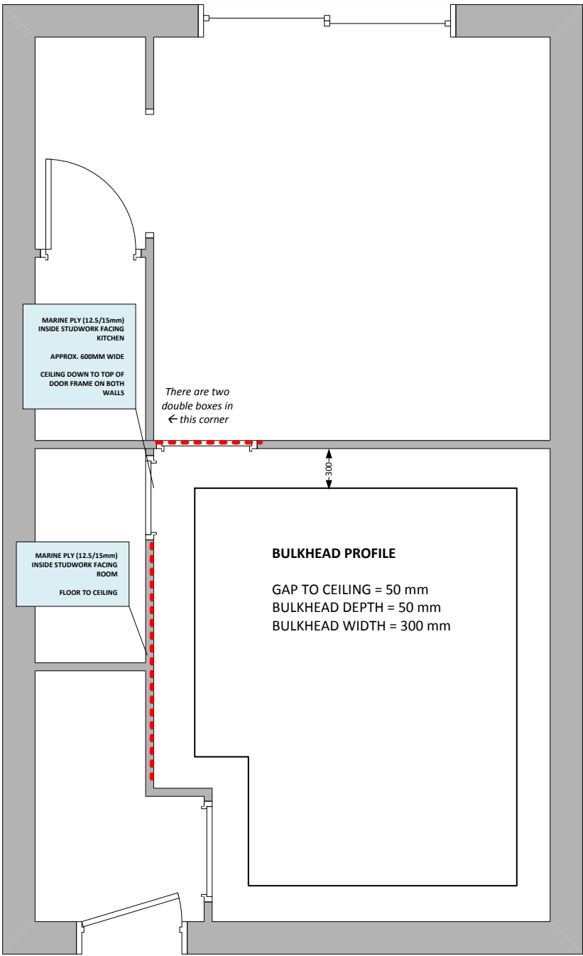
PLOT 35 APPENDIX C – DRYLINING – GROUND FLOOR v1.7 SNAGGING
