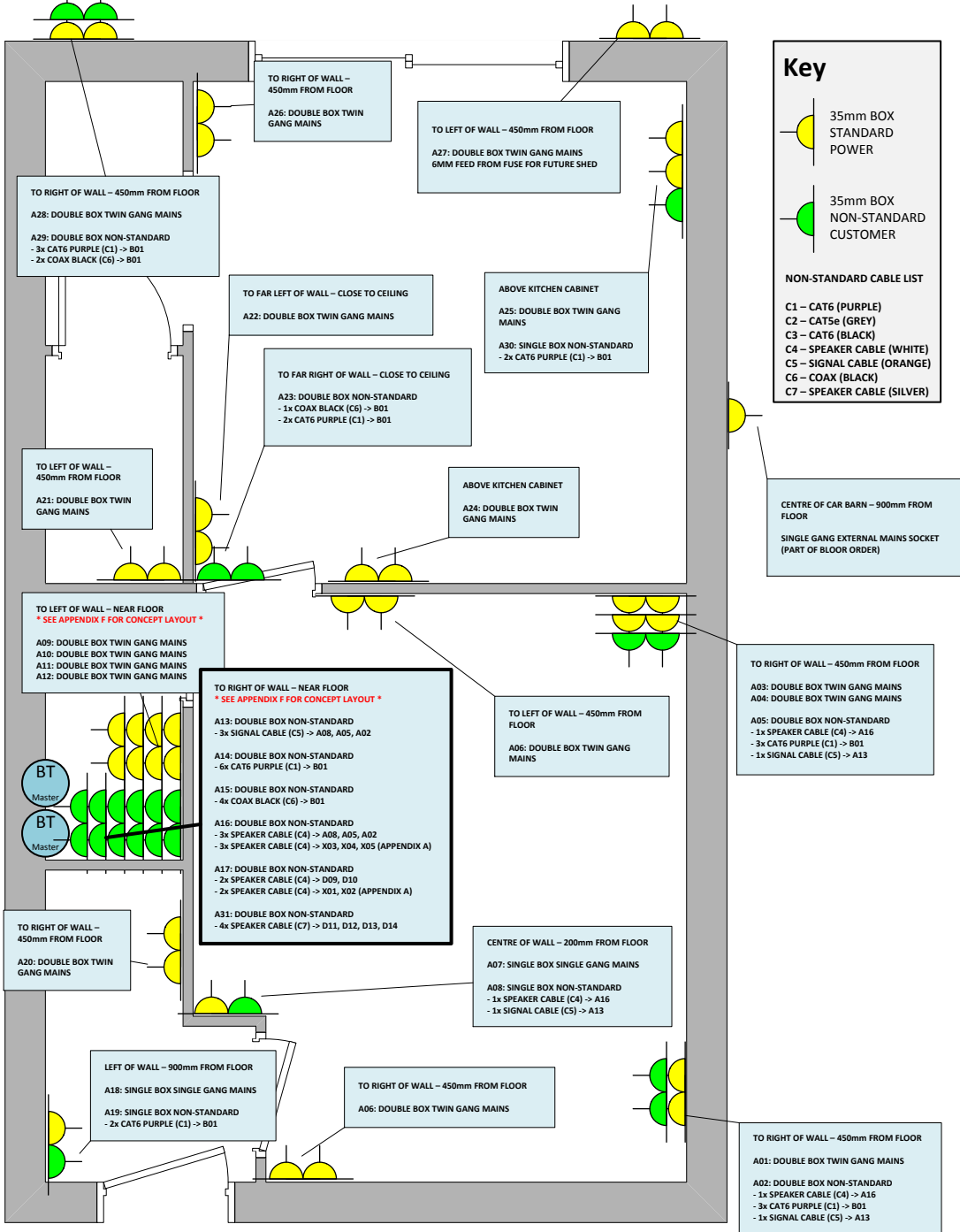
PLOT 35 WALL BOXES/CABLE – GROUND FLOOR v1.7 SNAGGING
