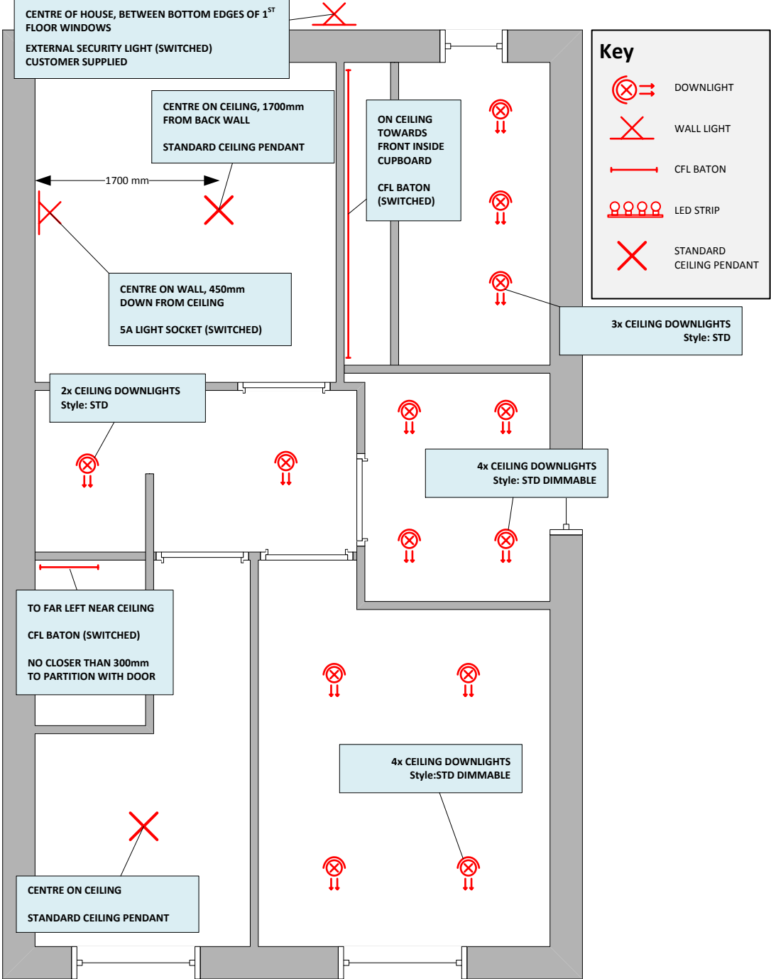
PLOT 35 LIGHTING – FIRST FLOOR v1.7 SNAGGING
