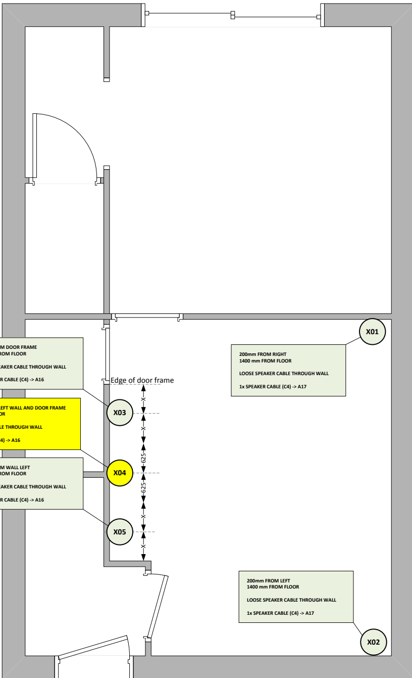
PLOT 35 APPENDIX A – LIVING ROOM SPEAKER LOCATIONS v1.7 SNAGGING
