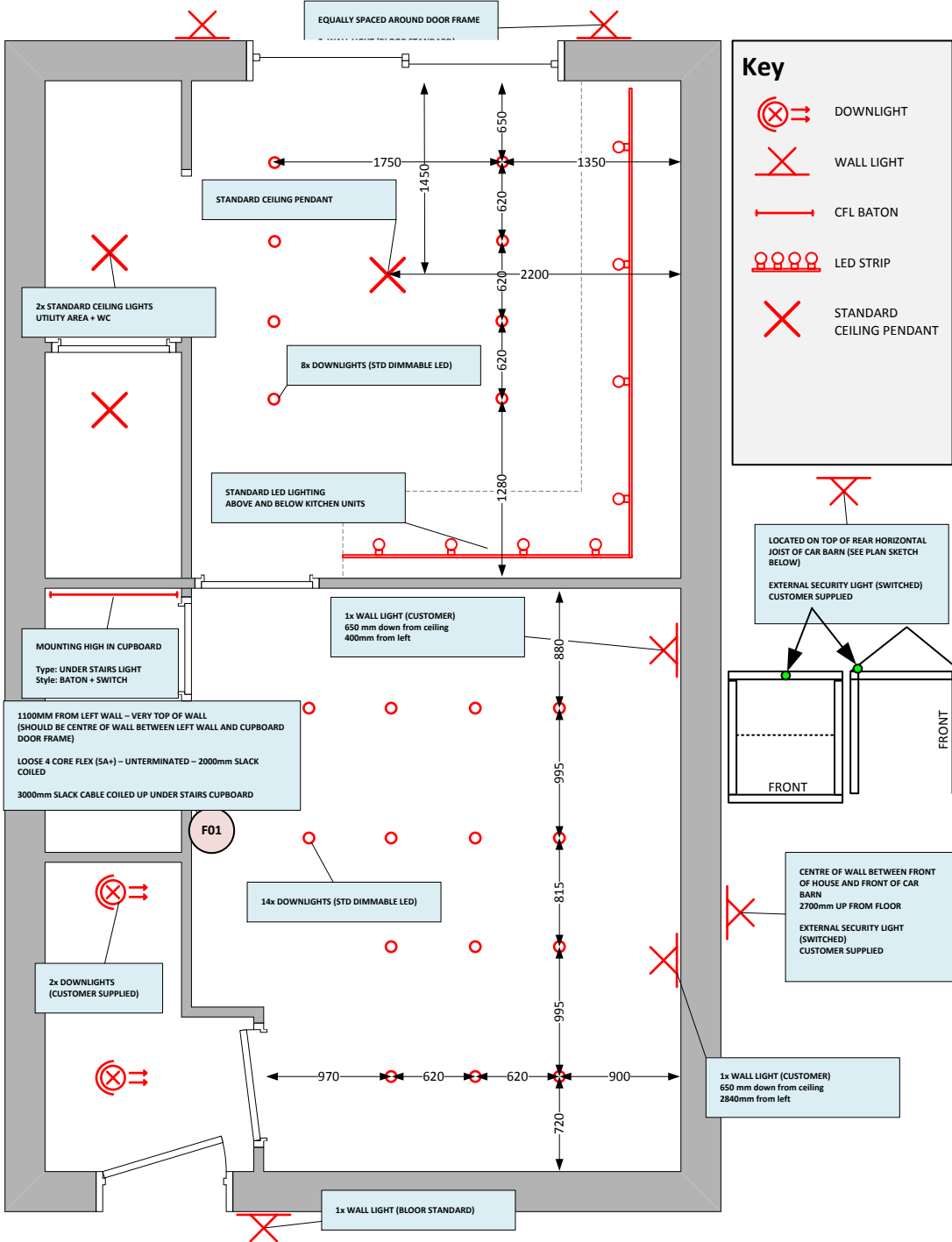
PLOT 35 LIGHTING – GROUND FLOOR v1.7 SNAGGING
